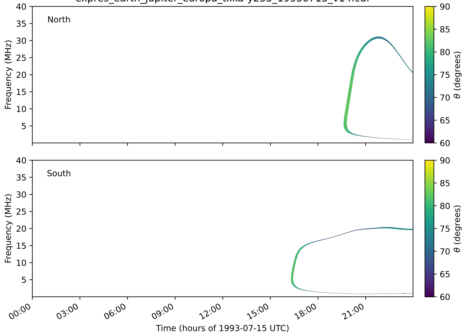
expres_earth_jupiter_europa_txka-y235_19930715_v14.cdf
