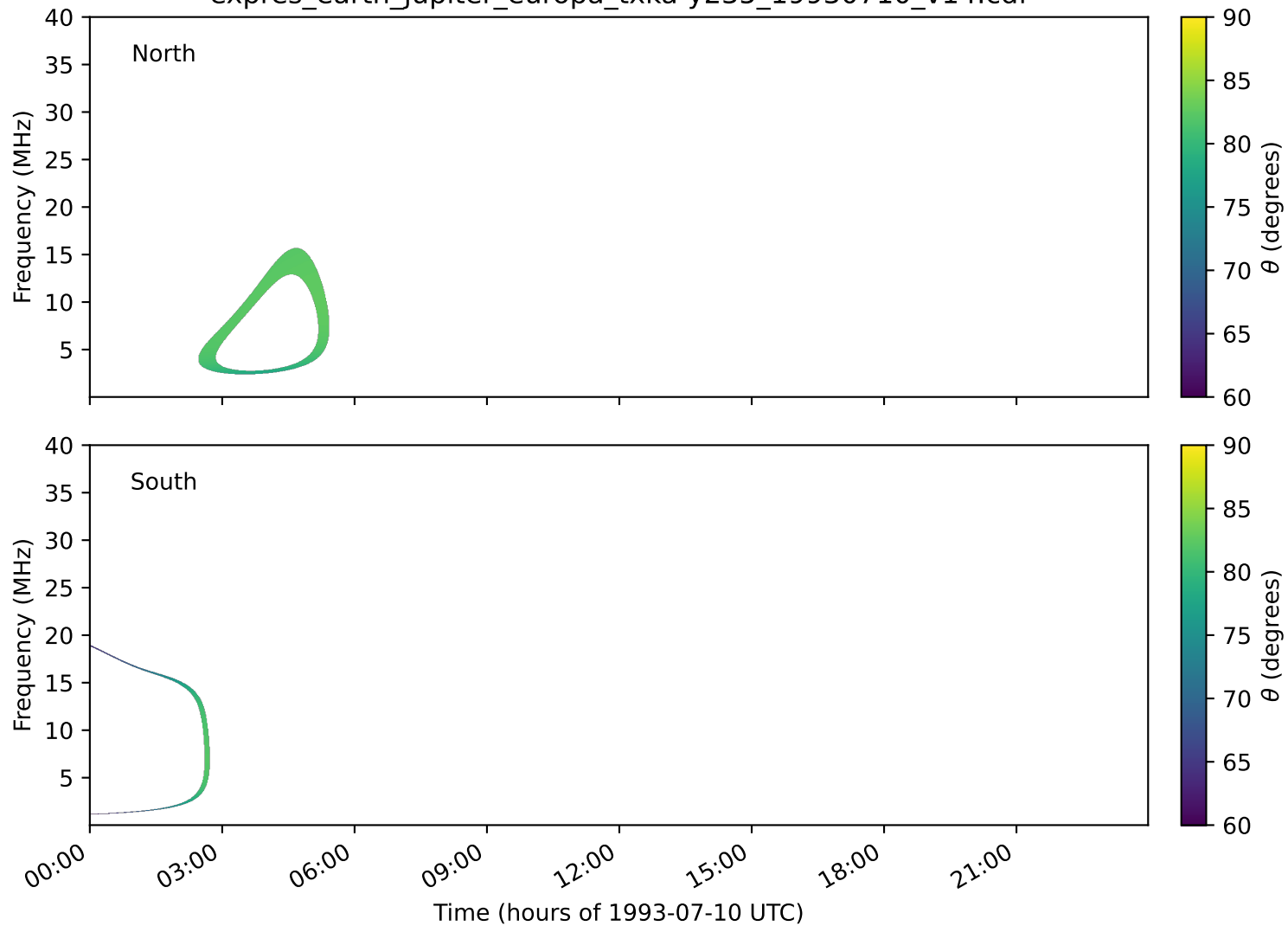
expres_earth_jupiter_europa_txka-y235_19930710_v14.cdf
