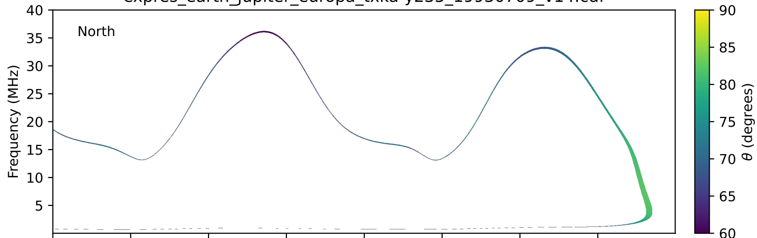
expres_earth_jupiter_europa_txka-y235_19930709_v14.cdf
