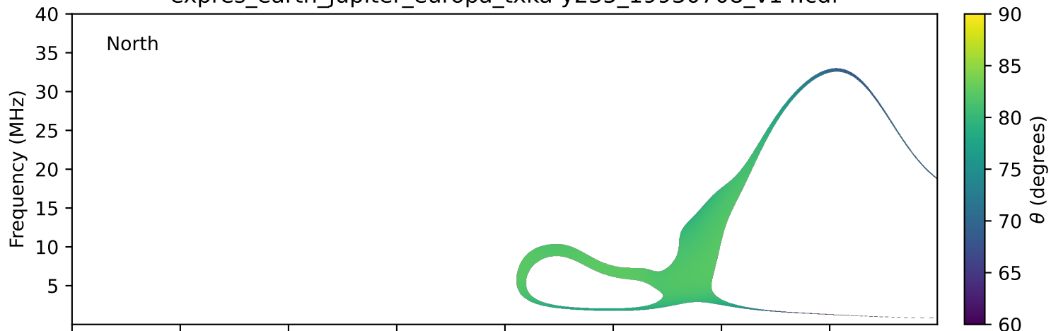
expres_earth_jupiter_europa_txka-y235_19930708_v14.cdf
