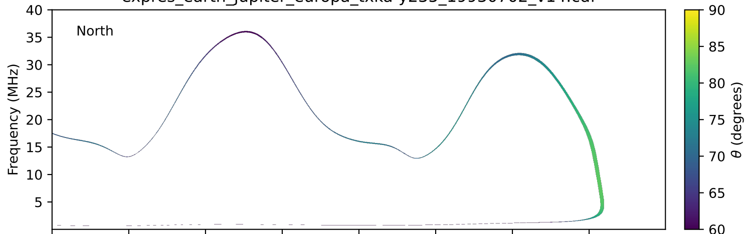
expres_earth_jupiter_europa_txka-y235_19930702_v14.cdf
