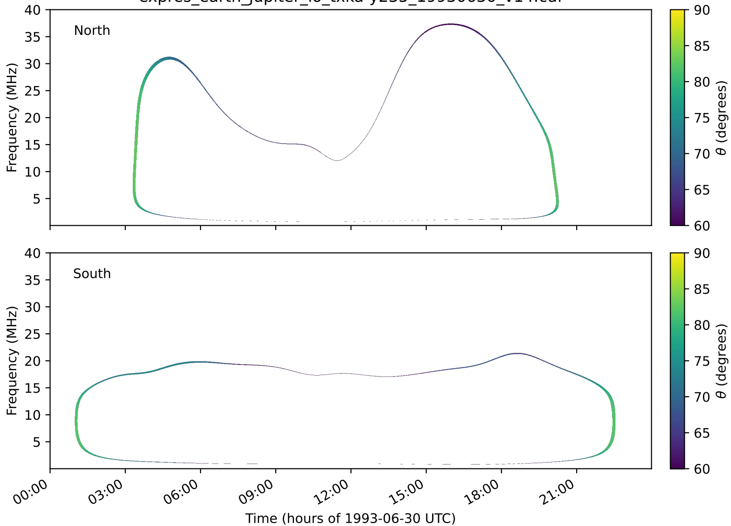
expres_earth_jupiter_io_txka-y235_19930630_v14.cdf
