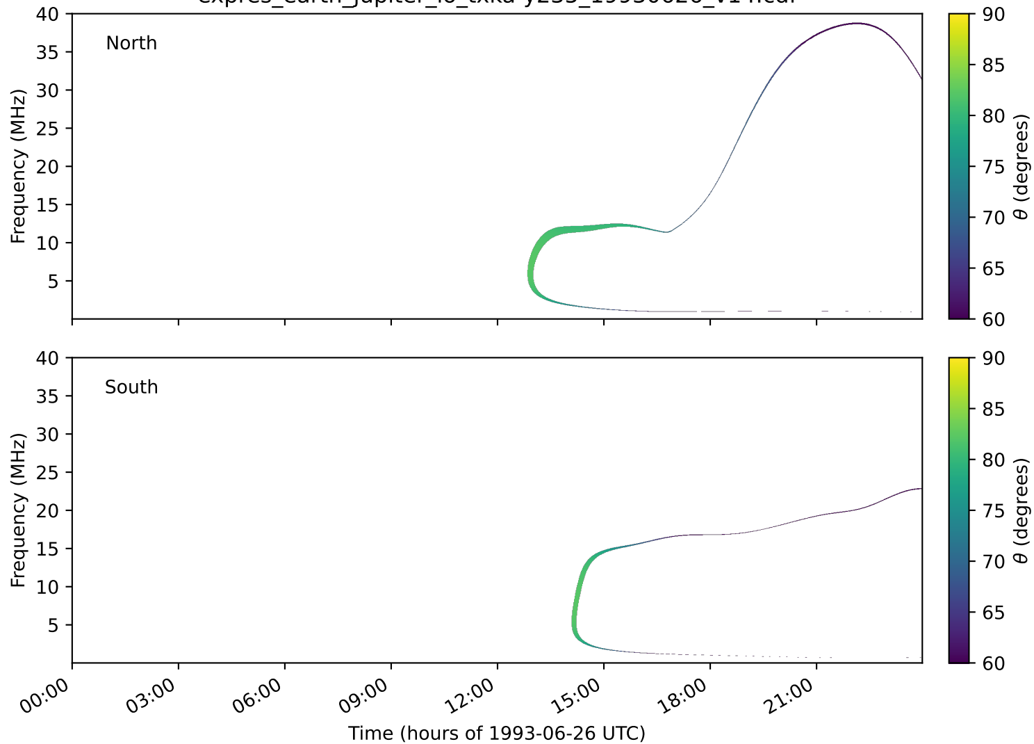
expres_earth_jupiter_io_txka-y235_19930626_v14.cdf
