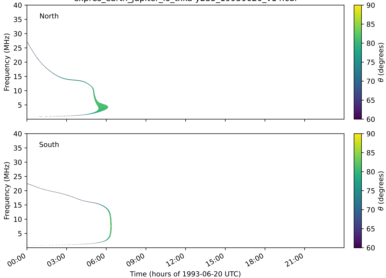
expres_earth_jupiter_io_txka-y235_19930620_v14.cdf
