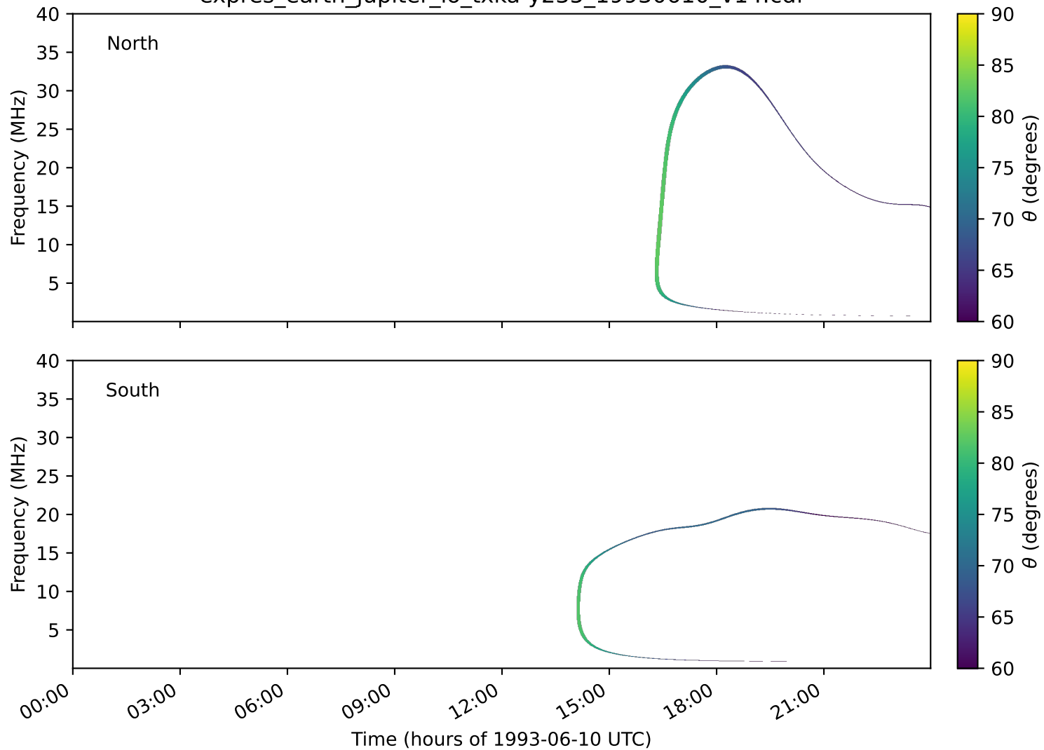
expres_earth_jupiter_io_txka-y235_19930610_v14.cdf
