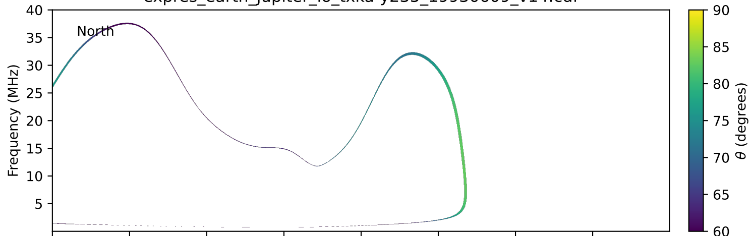
expres_earth_jupiter_io_txka-y235_19930609_v14.cdf
