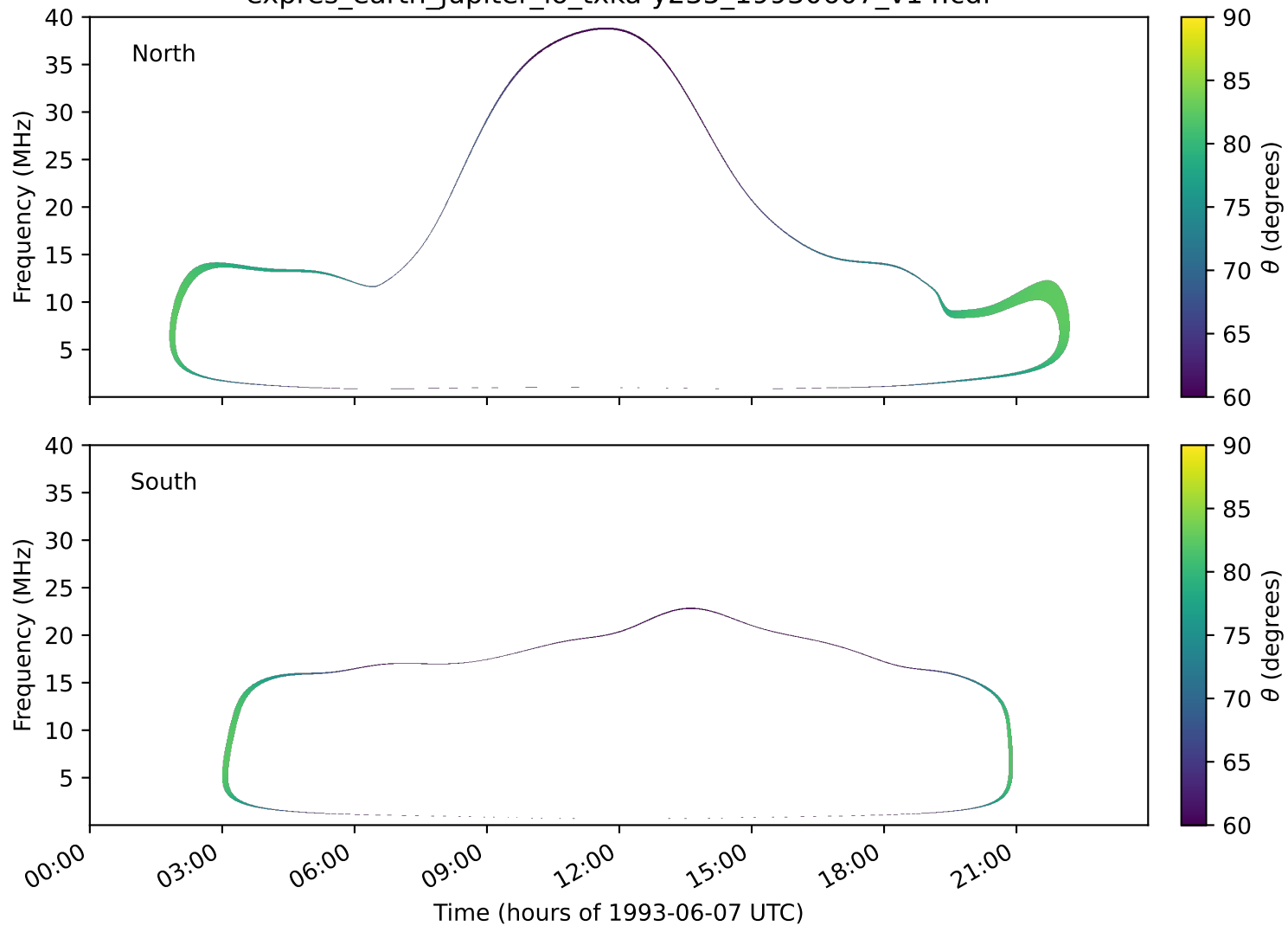
expres_earth_jupiter_io_txka-y235_19930607_v14.cdf
