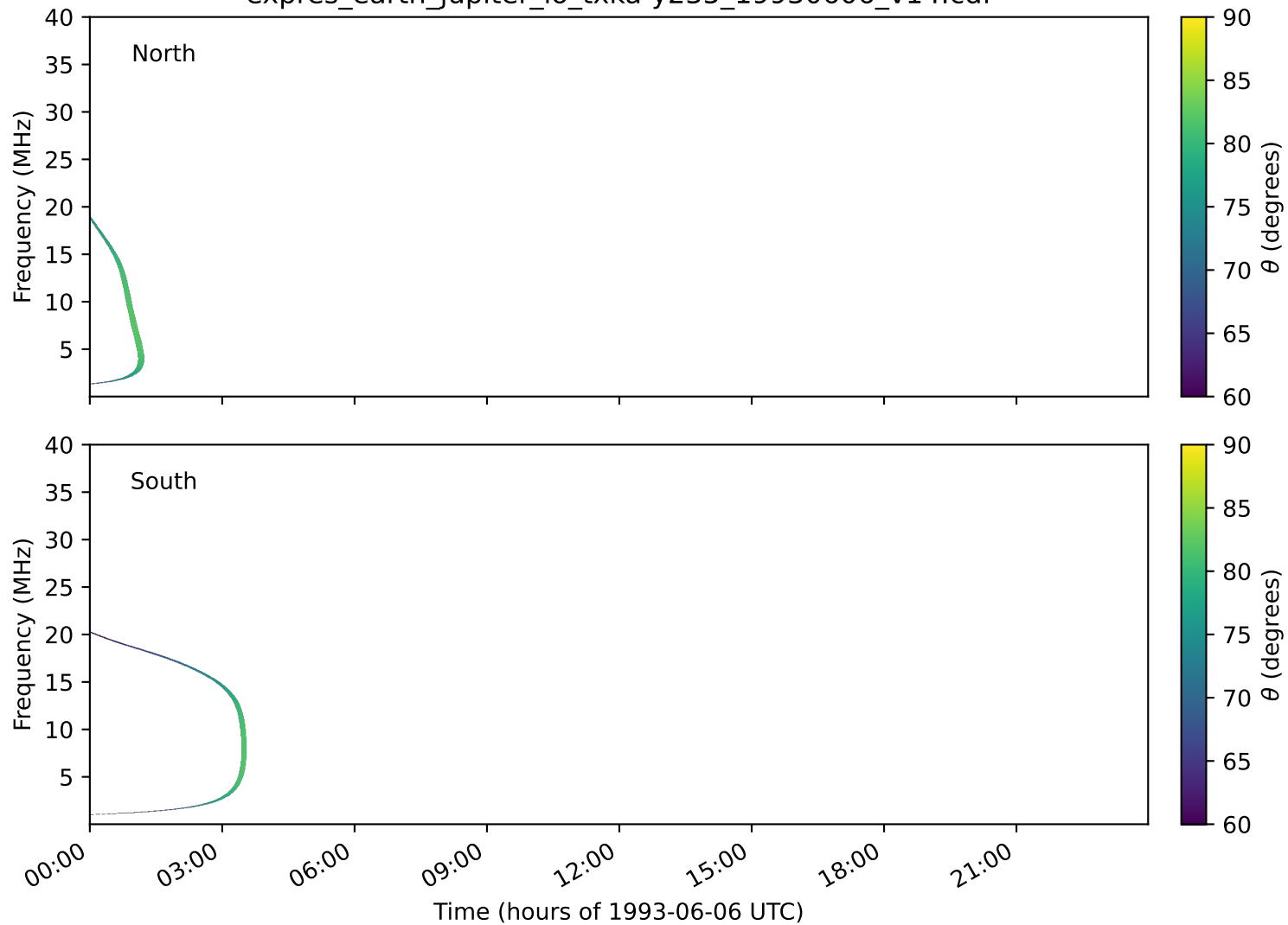
expres_earth_jupiter_io_txka-y235_19930606_v14.cdf
