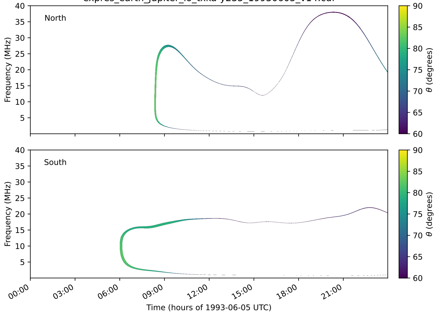
expres_earth_jupiter_io_txka-y235_19930605_v14.cdf
