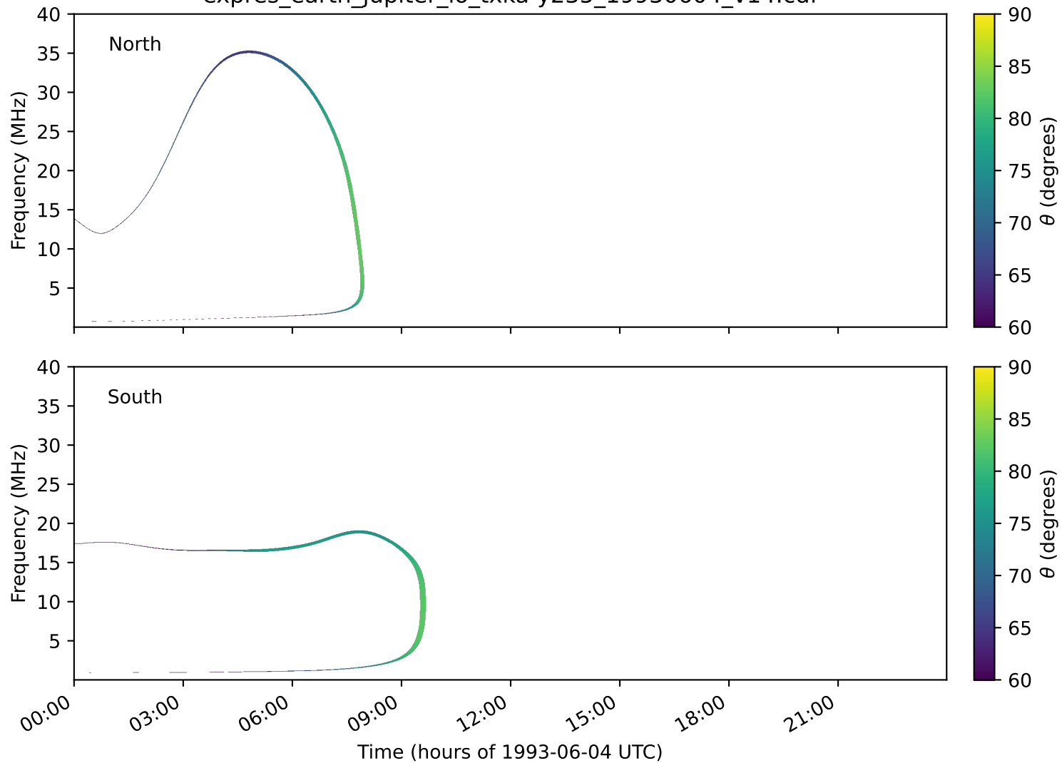
expres_earth_jupiter_io_txka-y235_19930604_v14.cdf
