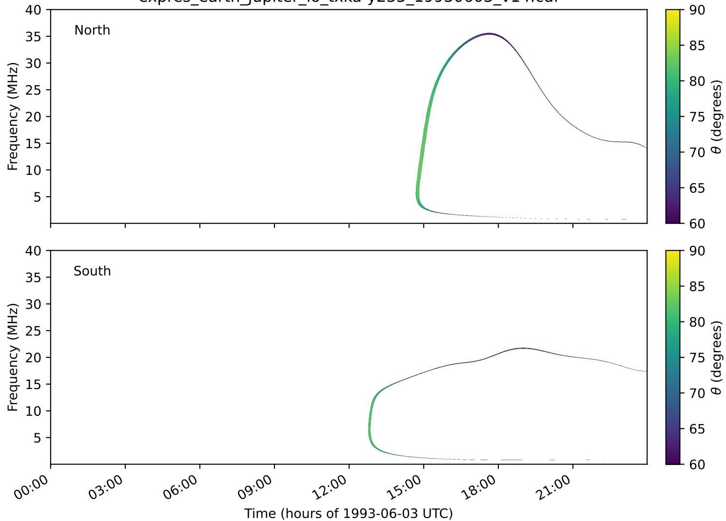
expres_earth_jupiter_io_txka-y235_19930603_v14.cdf
