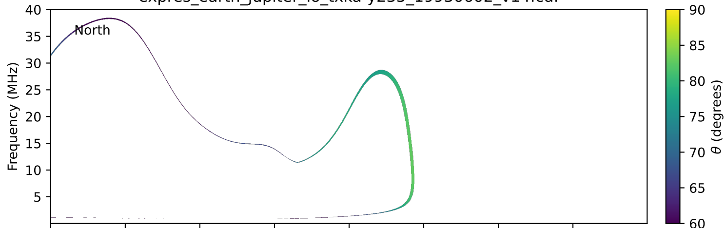
expres_earth_jupiter_io_txka-y235_19930602_v14.cdf
