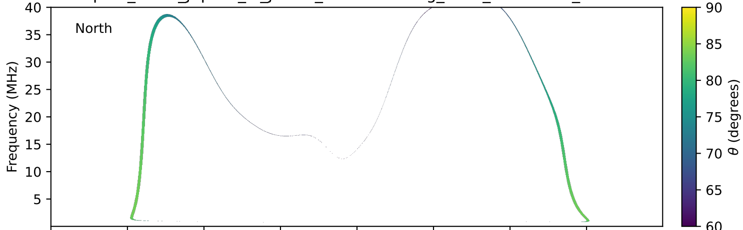
expres_earth_jupiter_io_jrm33_lossc-wid1deg_3kev_19930630_v11.cdf
