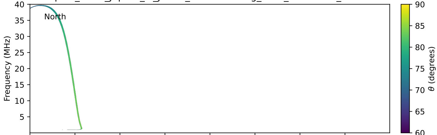
expres_earth_jupiter_io_jrm33_lossc-wid1deg_3kev_19930629_v11.cdf
