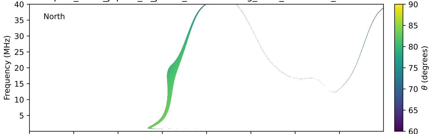
expres_earth_jupiter_io_jrm33_lossc-wid1deg_3kev_19930628_v11.cdf
