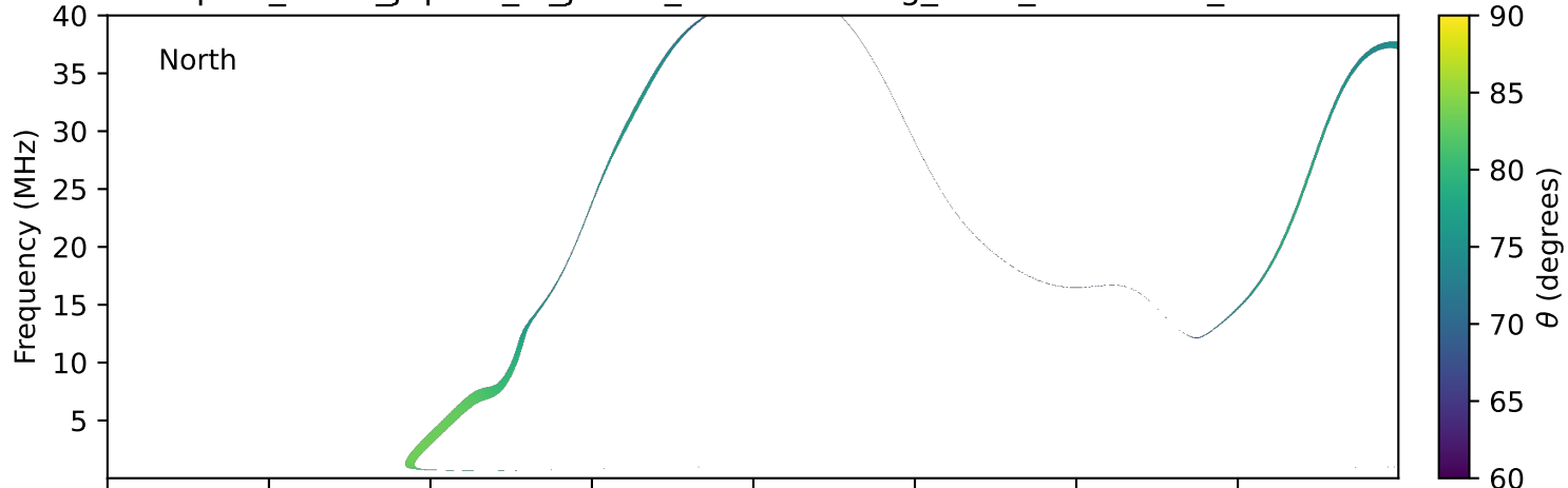
expres_earth_jupiter_io_jrm33_lossc-wid1deg_3kev_19930621_v11.cdf
