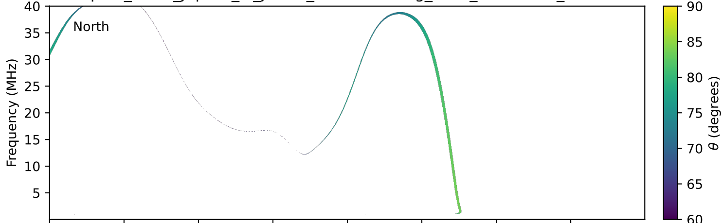
expres_earth_jupiter_io_jrm33_lossc-wid1deg_3kev_19930609_v11.cdf
