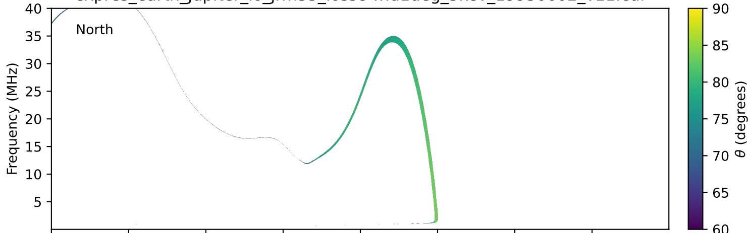
expres_earth_jupiter_io_jrm33_lossc-wid1deg_3kev_19930602_v11.cdf
