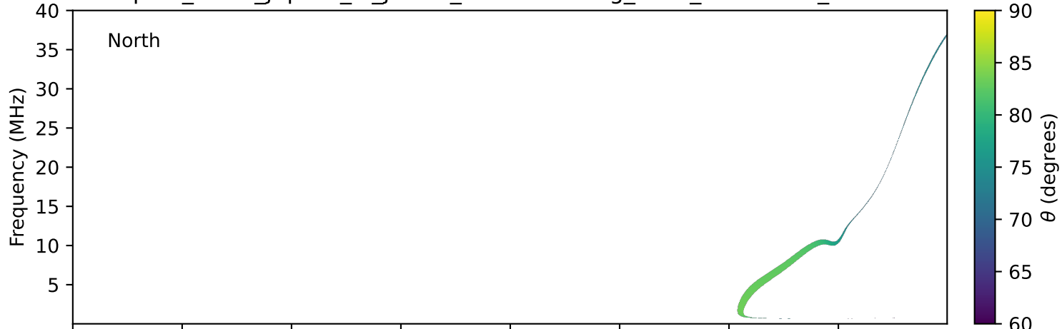
expres_earth_jupiter_io_jrm33_lossc-wid1deg_3kev_19930601_v11.cdf
