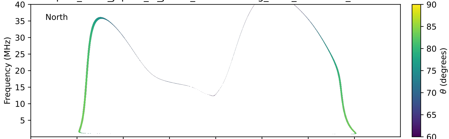
expres_earth_jupiter_io_jrm09_lossc-wid1deg_3kev_19930630_v11.cdf
