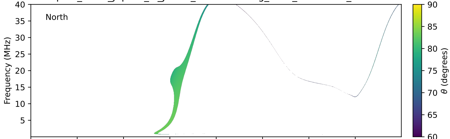
expres_earth_jupiter_io_jrm09_lossc-wid1deg_3kev_19930628_v11.cdf
