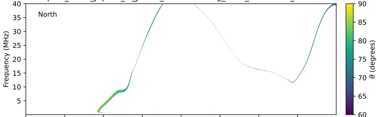
expres_earth_jupiter_io_jrm09_lossc-wid1deg_3kev_19930621_v11.cdf
