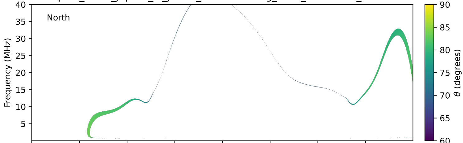
expres_earth_jupiter_io_jrm09_lossc-wid1deg_3kev_19930614_v11.cdf
