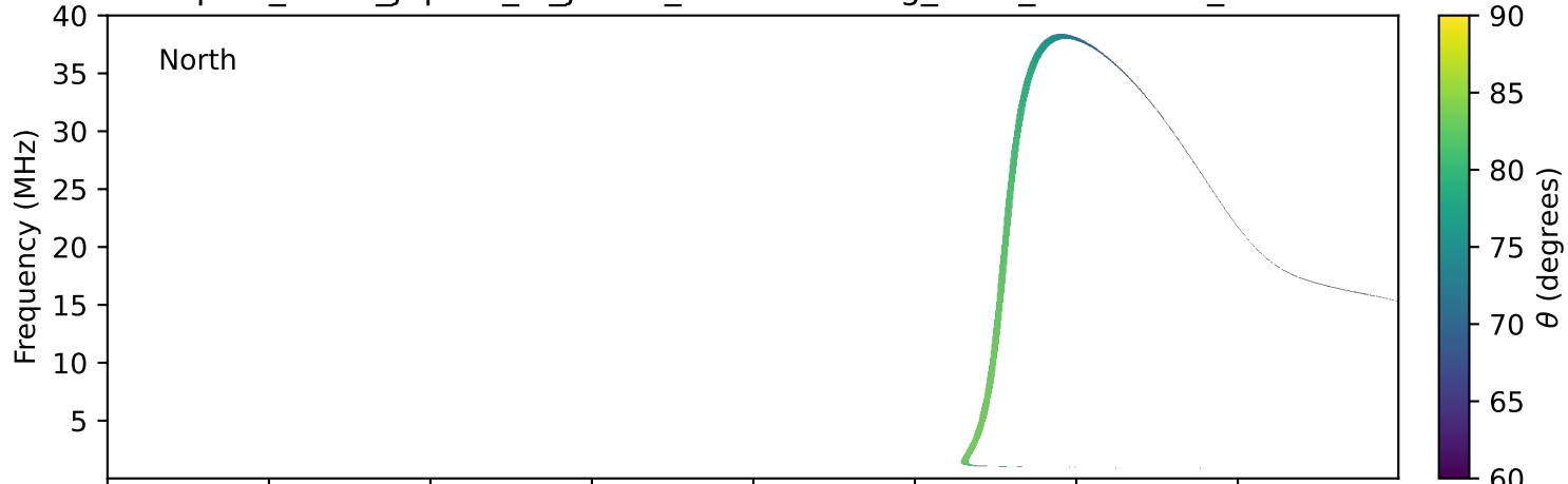
expres_earth_jupiter_io_jrm09_lossc-wid1deg_3kev_19930610_v11.cdf
