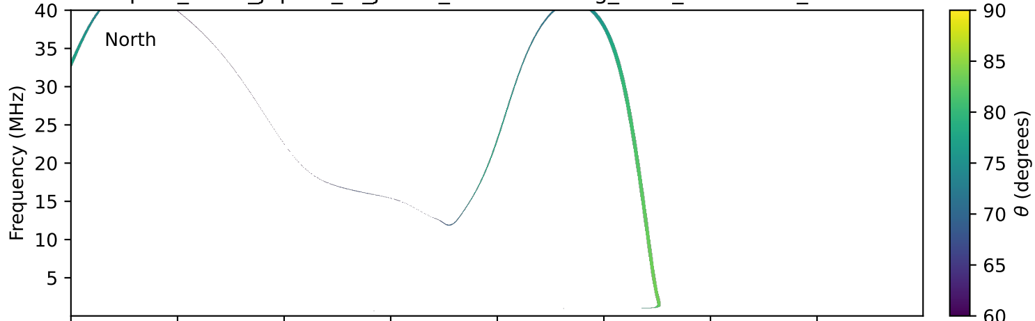
expres_earth_jupiter_io_jrm09_lossc-wid1deg_3kev_19930609_v11.cdf
