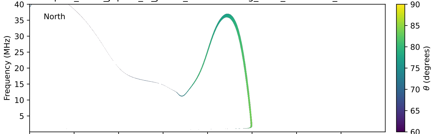
expres_earth_jupiter_io_jrm09_lossc-wid1deg_3kev_19930602_v11.cdf
