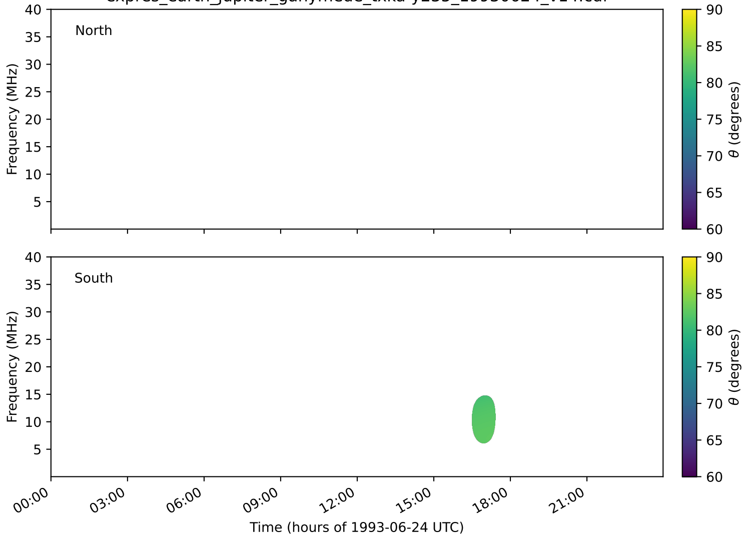
expres_earth_jupiter_ganymede_txka-y235_19930624_v14.cdf
