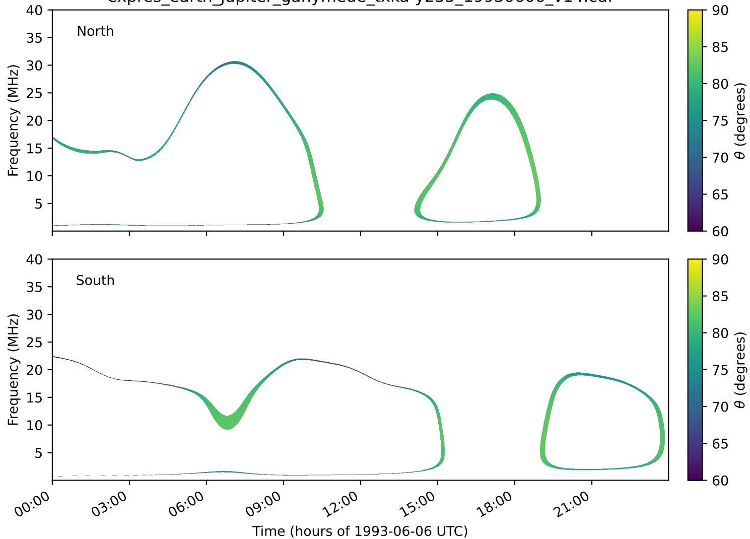
expres_earth_jupiter_ganymede_txka-y235_19930606_v14.cdf
