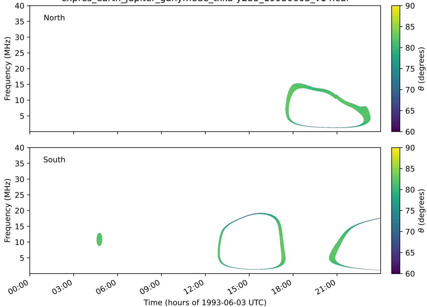
expres_earth_jupiter_ganymede_txka-y235_19930603_v14.cdf
