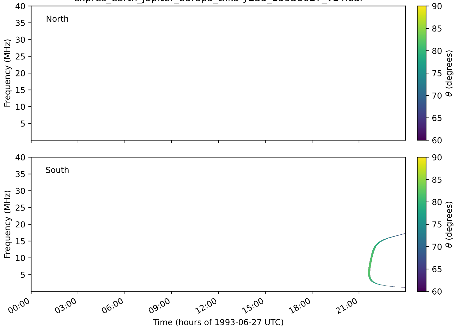
expres_earth_jupiter_europa_txka-y235_19930627_v14.cdf
