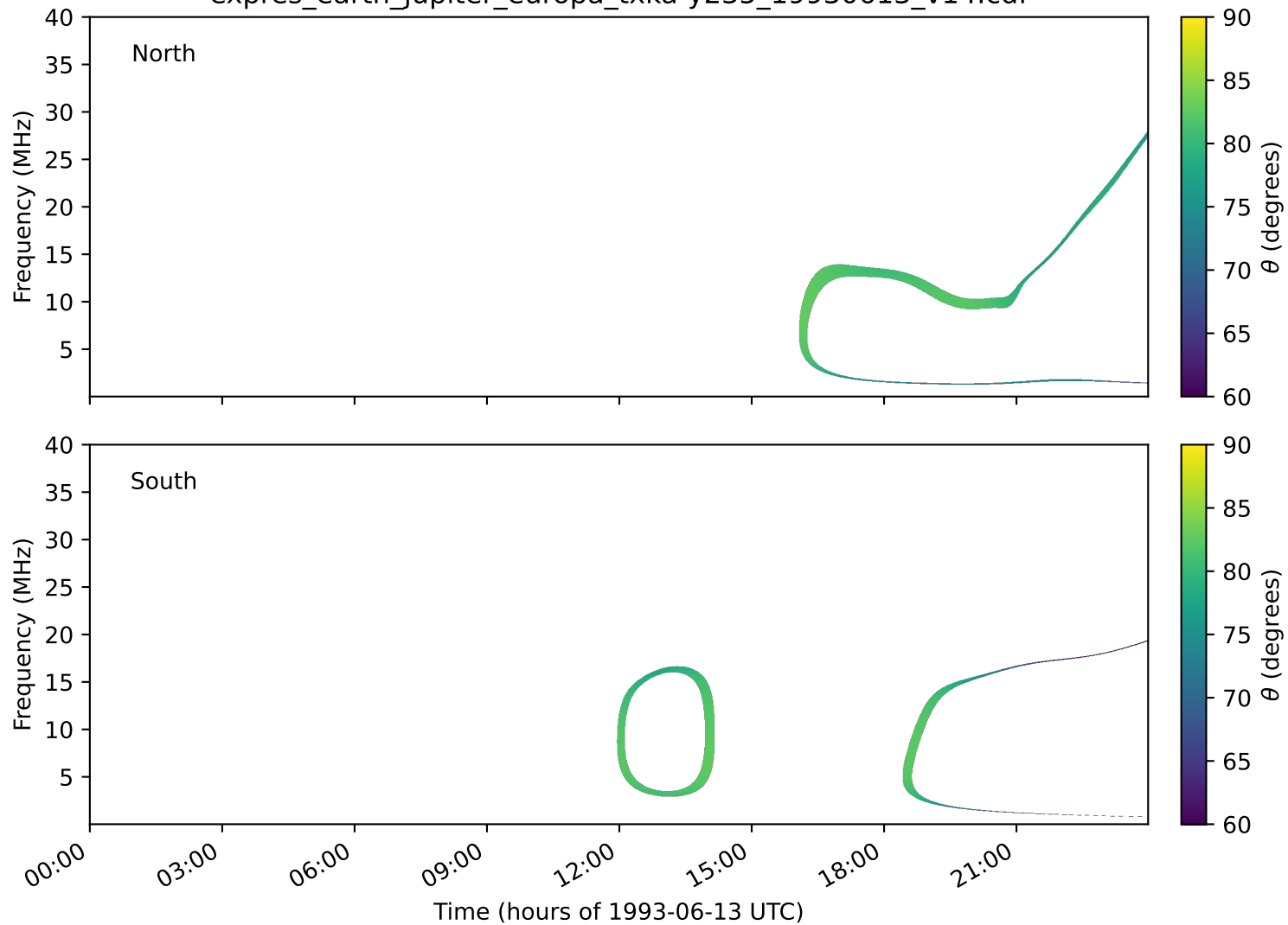
expres_earth_jupiter_europa_txka-y235_19930613_v14.cdf
