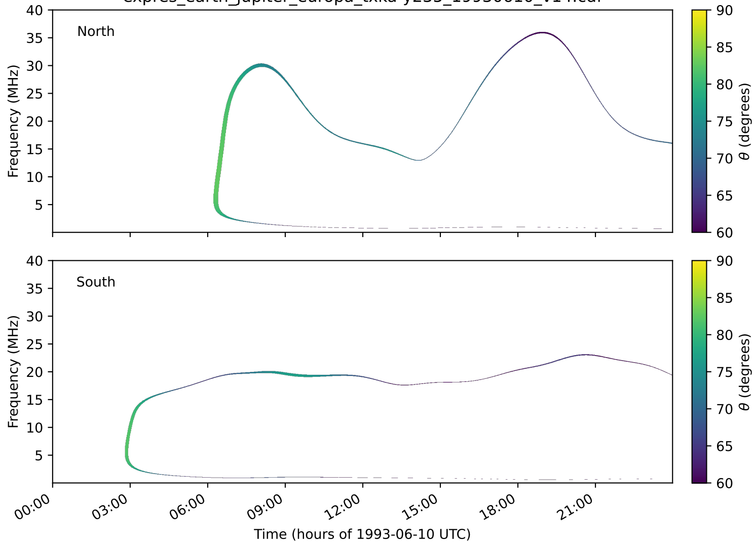
expres_earth_jupiter_europa_txka-y235_19930610_v14.cdf
