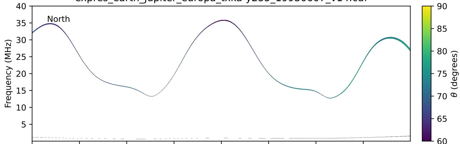
expres_earth_jupiter_europa_txka-y235_19930607_v14.cdf
