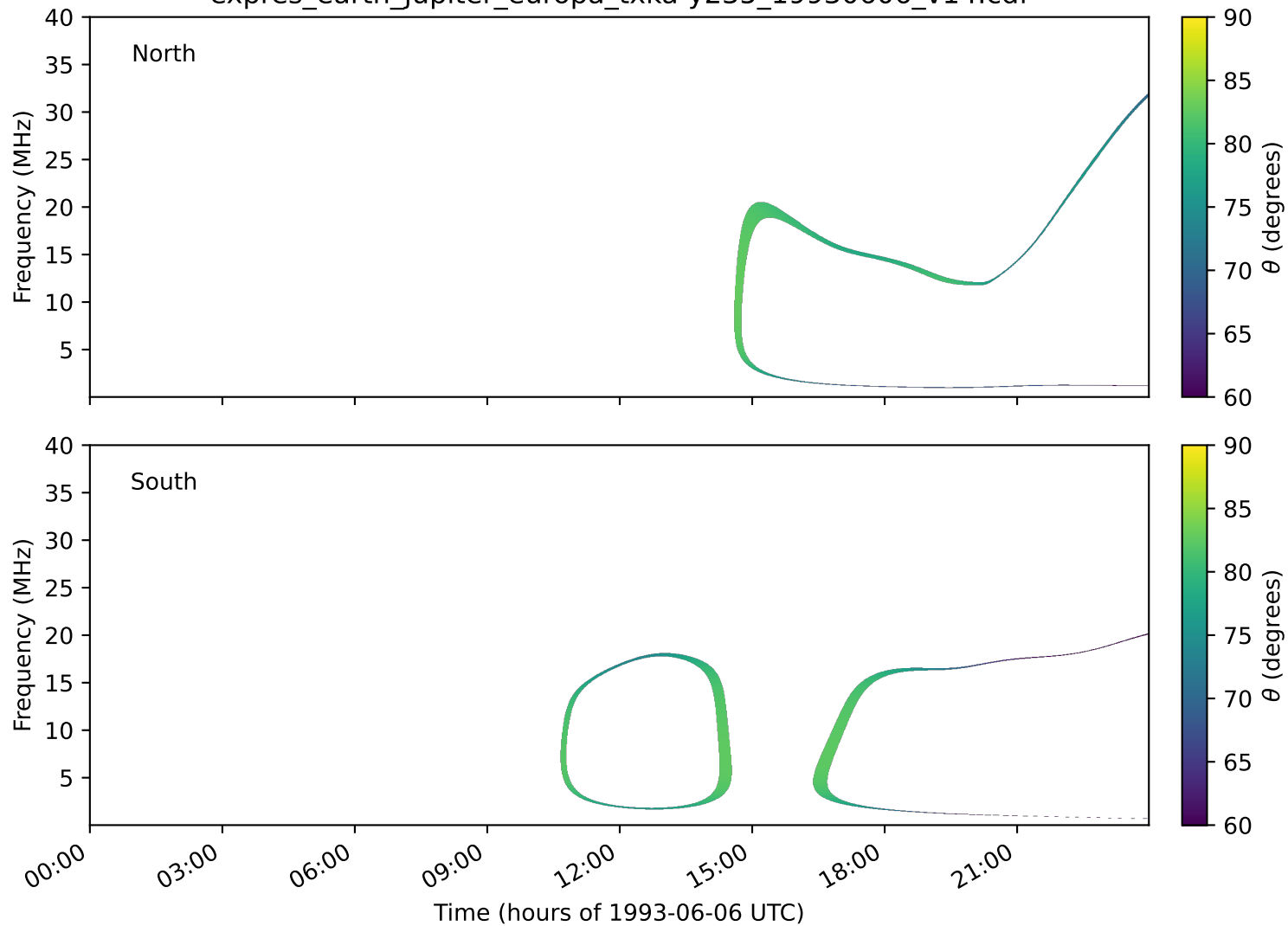
expres_earth_jupiter_europa_txka-y235_19930606_v14.cdf
