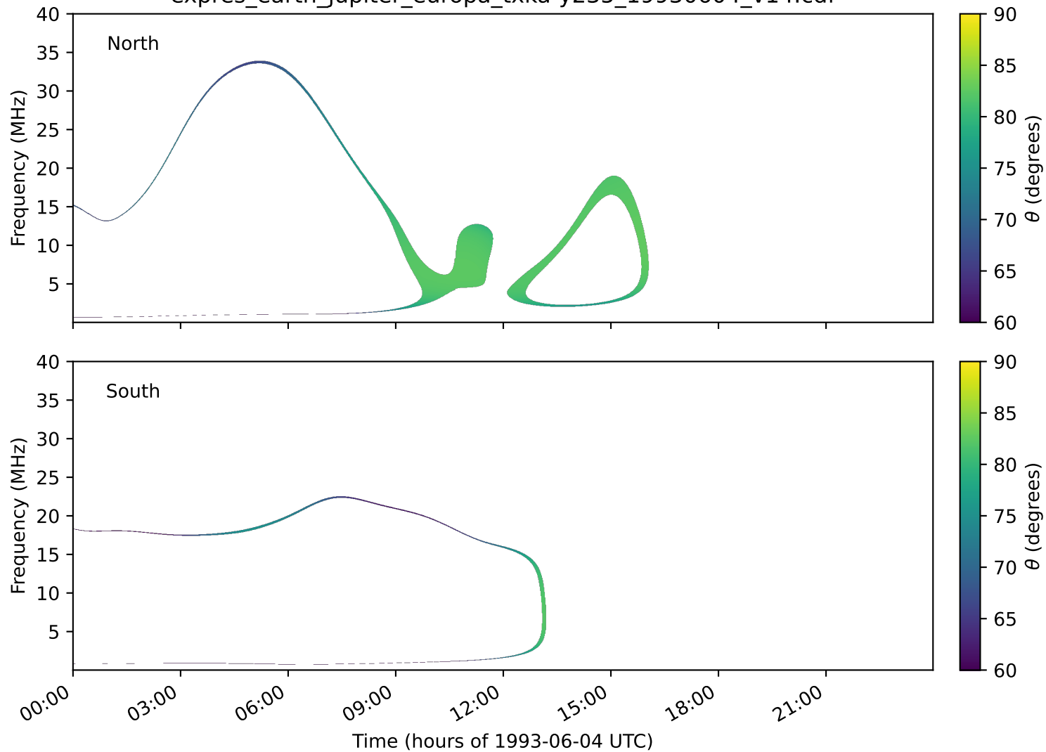
expres_earth_jupiter_europa_txka-y235_19930604_v14.cdf
