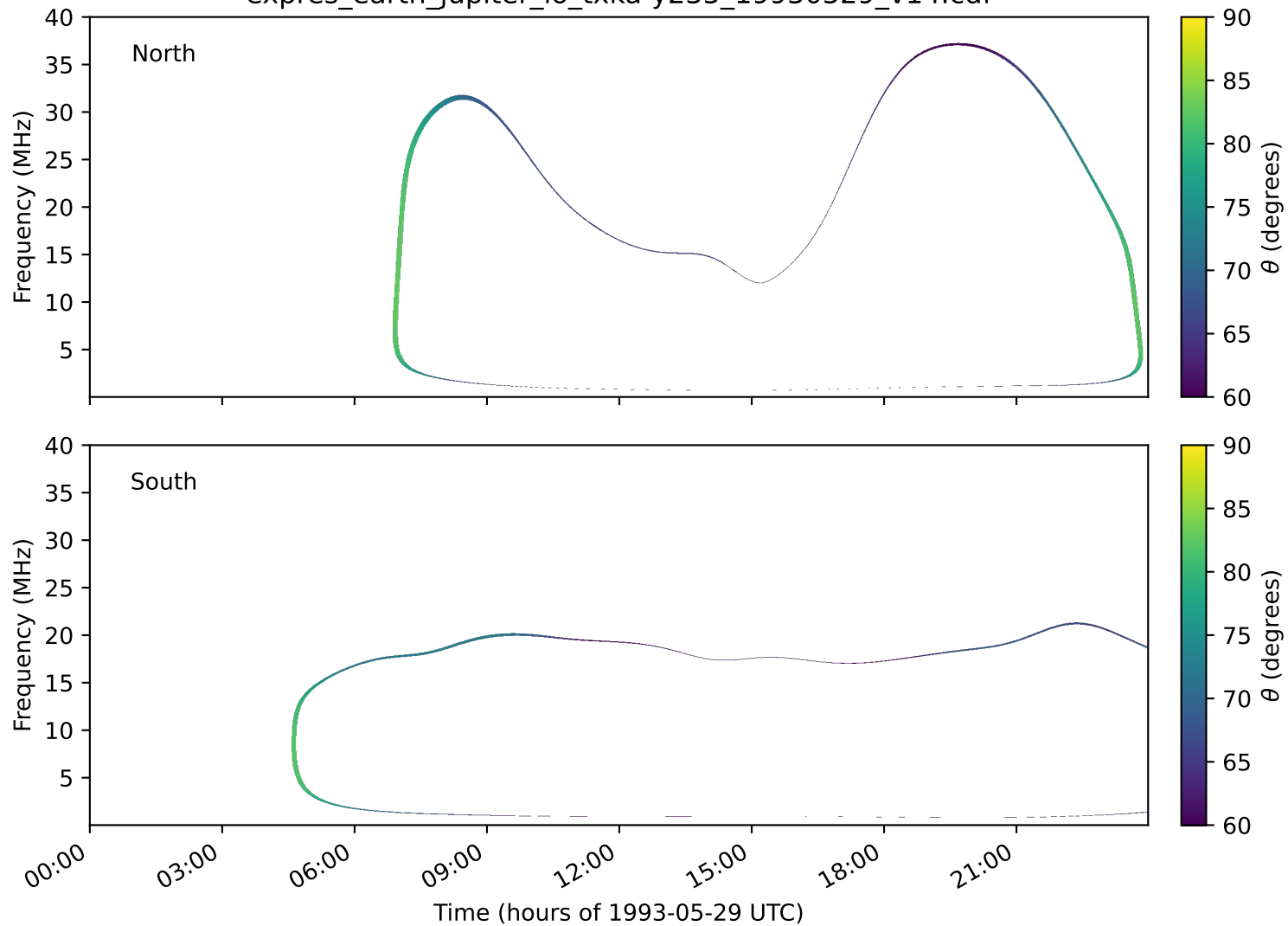
expres_earth_jupiter_io_txka-y235_19930529_v14.cdf
