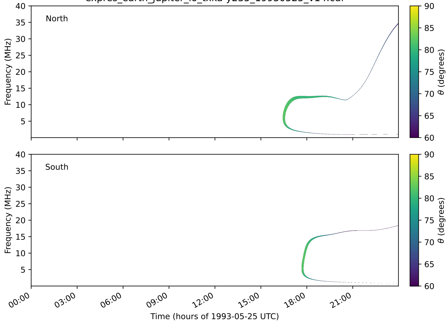
expres_earth_jupiter_io_txka-y235_19930525_v14.cdf
