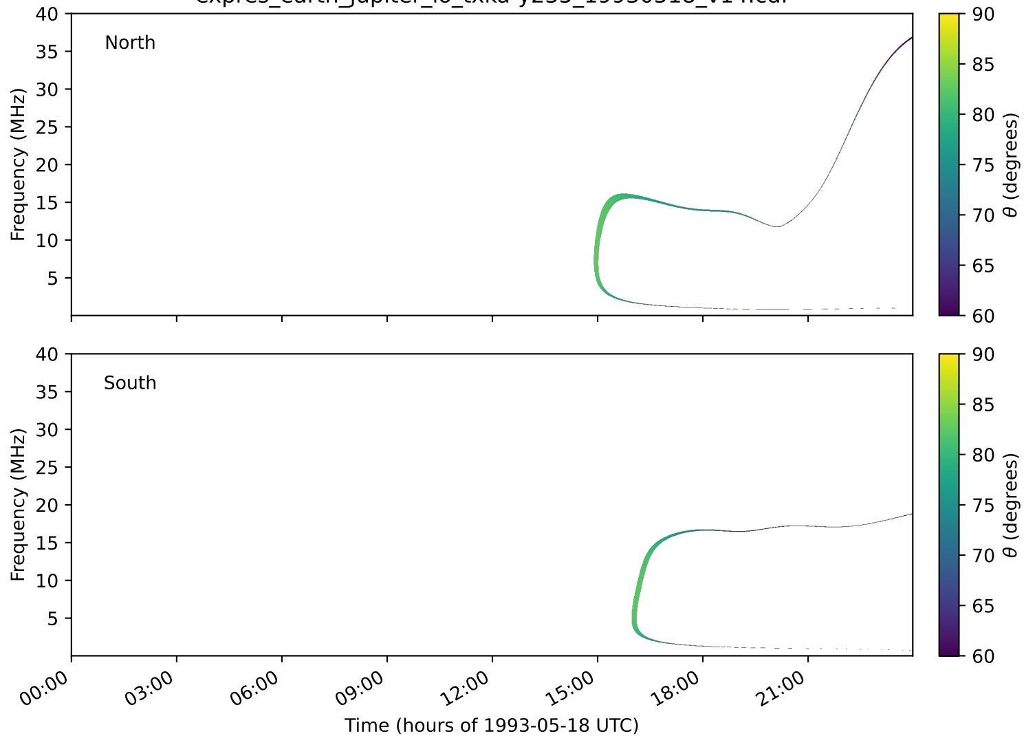
expres_earth_jupiter_io_txka-y235_19930518_v14.cdf
