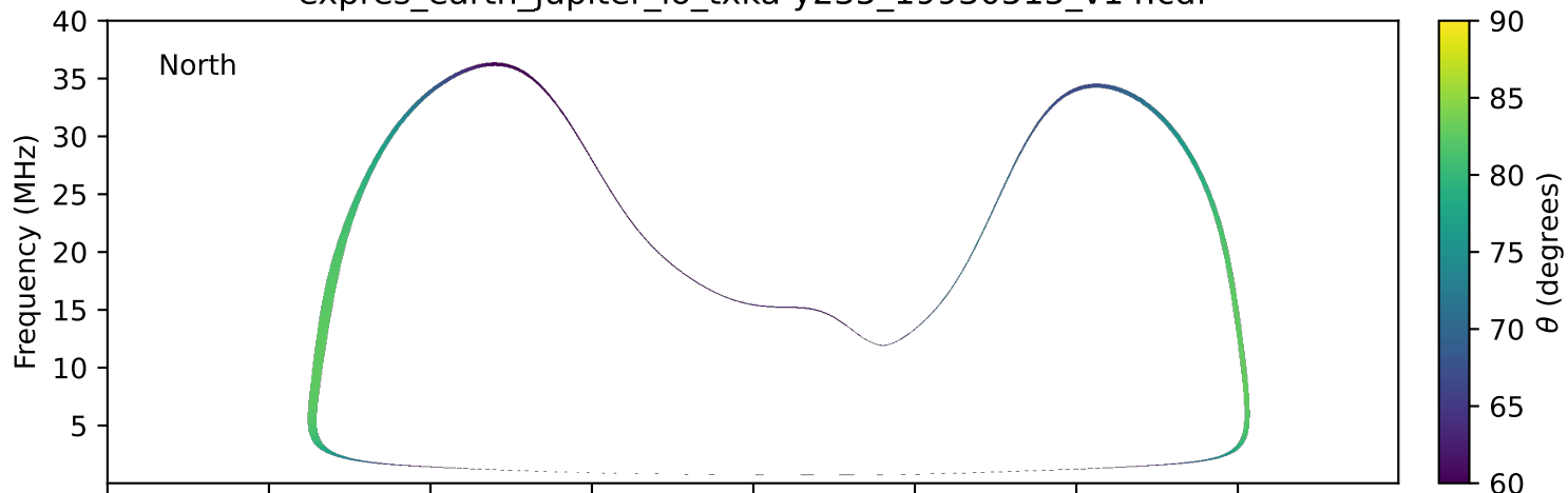
expres_earth_jupiter_io_txka-y235_19930515_v14.cdf
