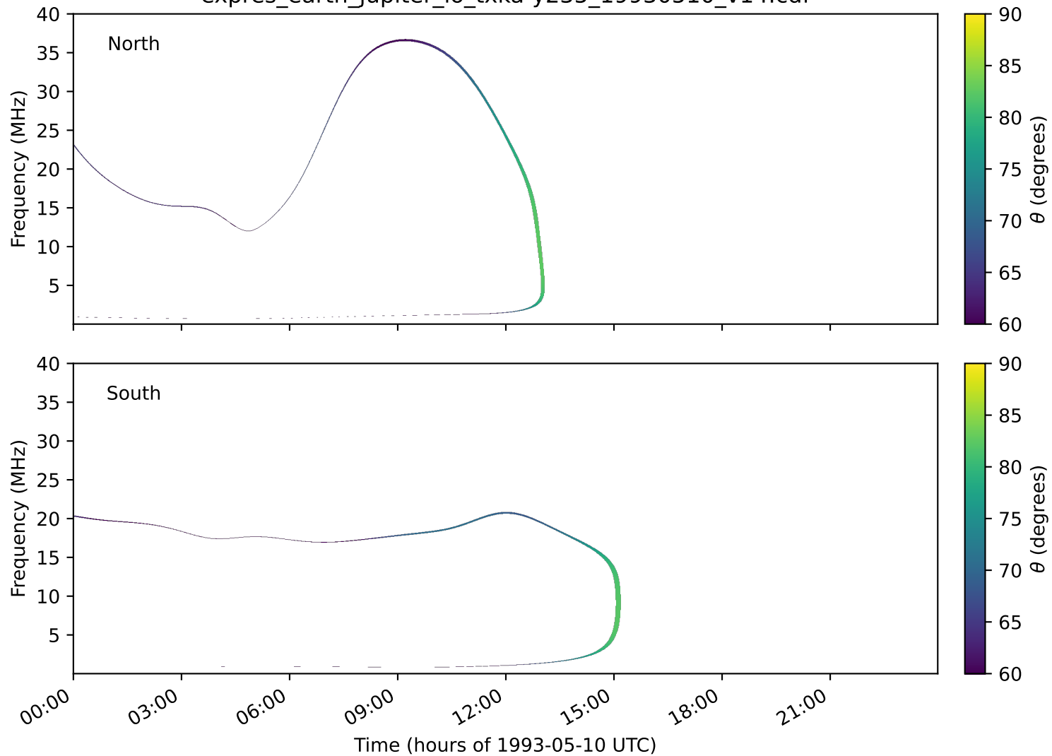
expres_earth_jupiter_io_txka-y235_19930510_v14.cdf
