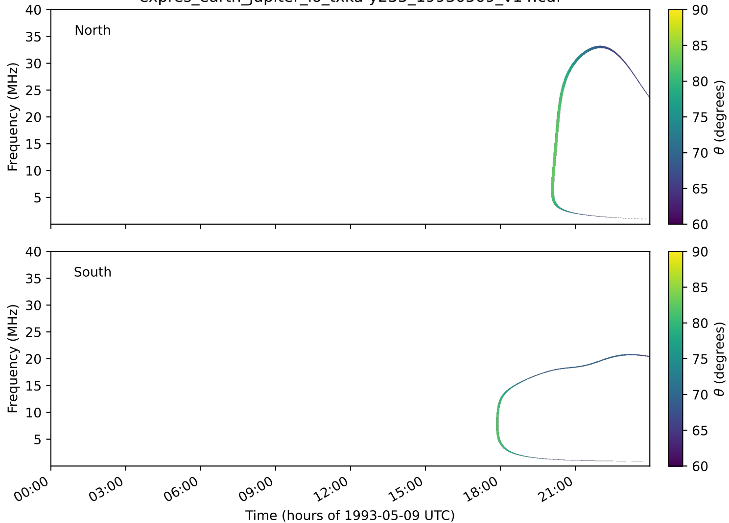
expres_earth_jupiter_io_txka-y235_19930509_v14.cdf
