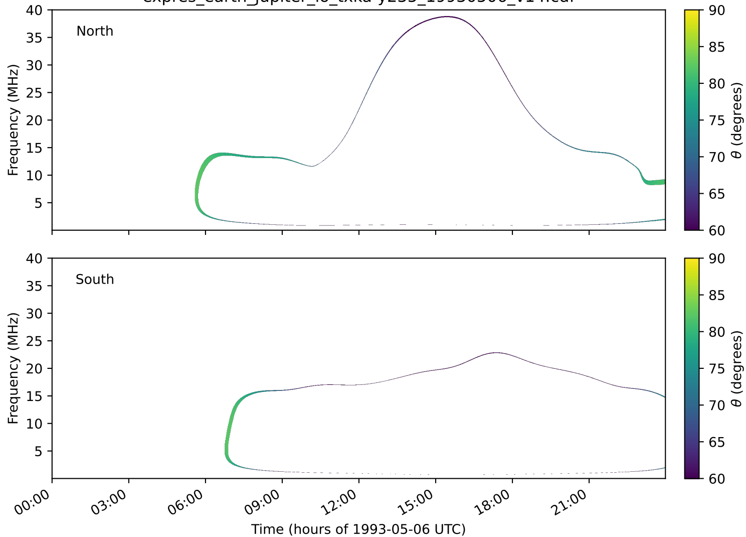
expres_earth_jupiter_io_txka-y235_19930506_v14.cdf
