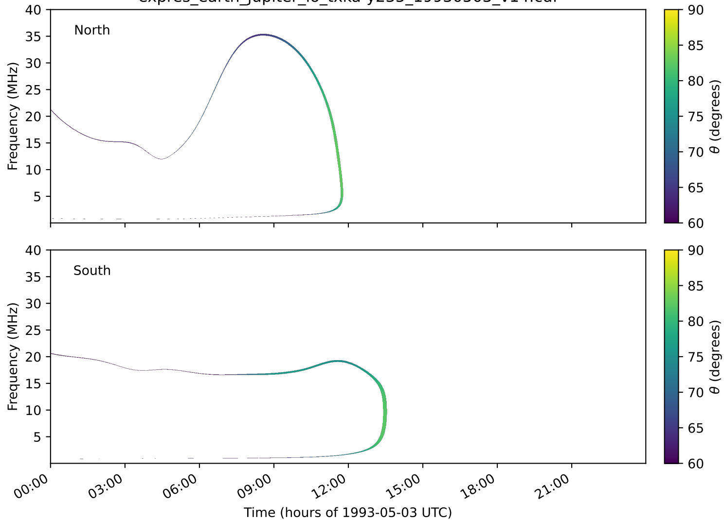
expres_earth_jupiter_io_txka-y235_19930503_v14.cdf
