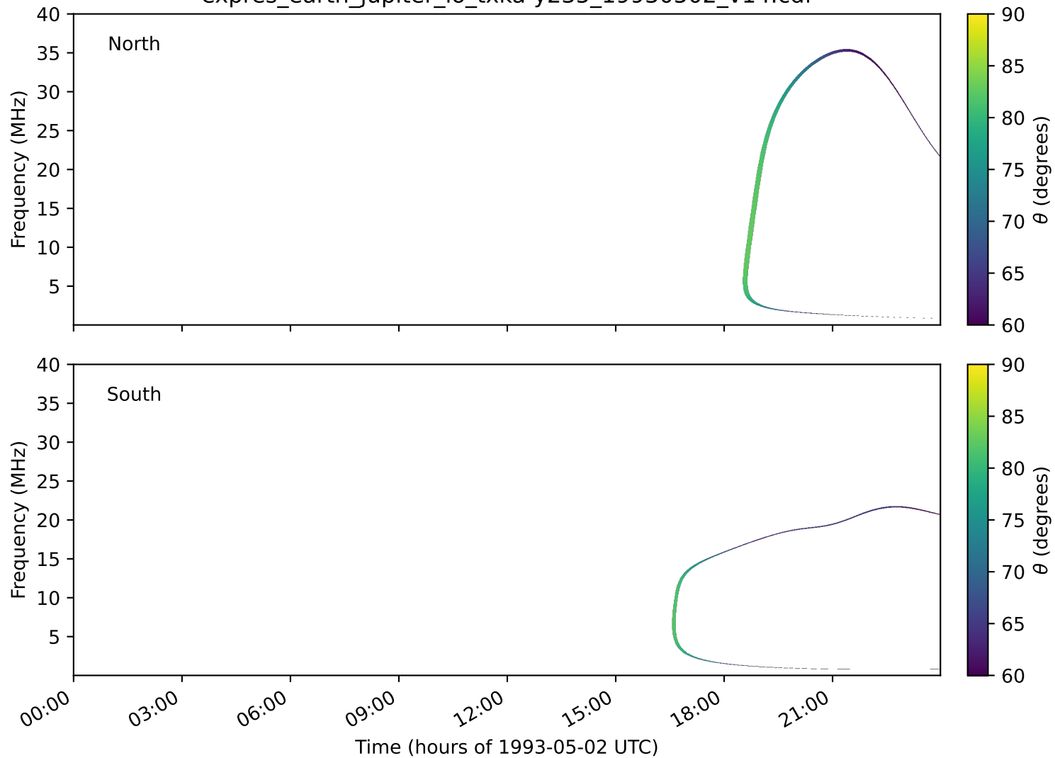
expres_earth_jupiter_io_txka-y235_19930502_v14.cdf
