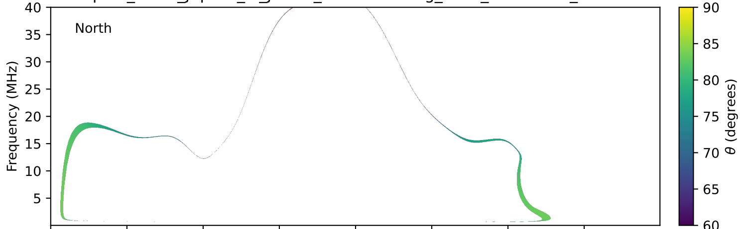
expres_earth_jupiter_io_jrm33_lossc-wid1deg_3kev_19930531_v11.cdf
