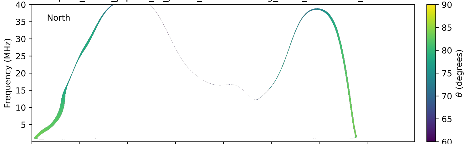
expres_earth_jupiter_io_jrm33_lossc-wid1deg_3kev_19930508_v11.cdf
